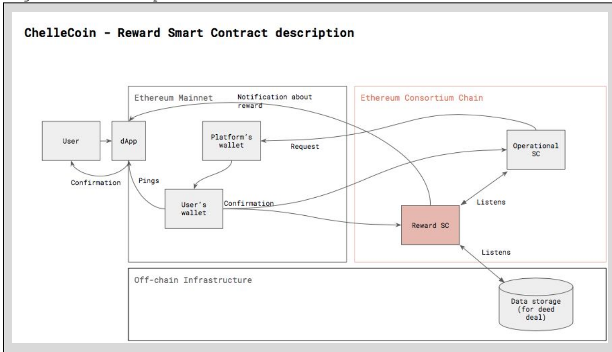
Figure 6. Description of the Chelle Reward Smart Contract
